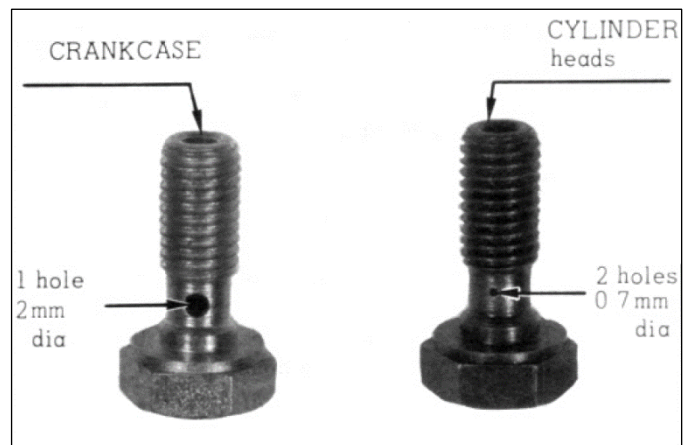
Fig. 5-6 Citroen 2CV Banjo Bolts
